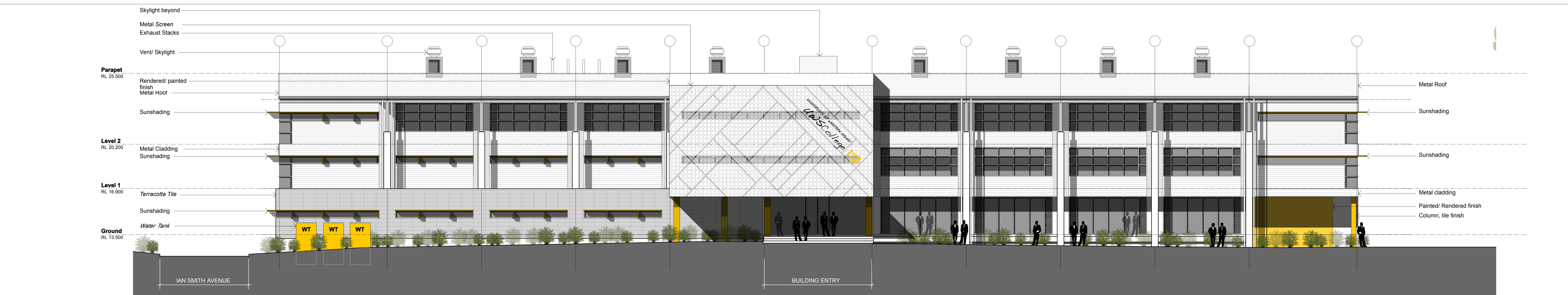
03 ELEVATION 3 - North UWSCollege Scale: 1:100 @ A0
