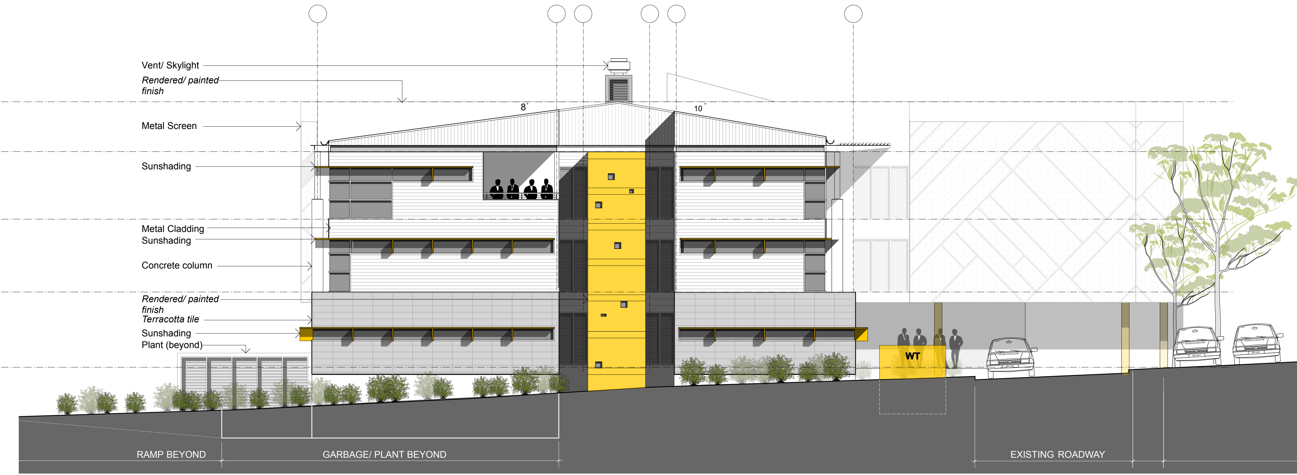
02 ELEVATION 2 - East UWSCollege Scale: 1:100 @ A0
